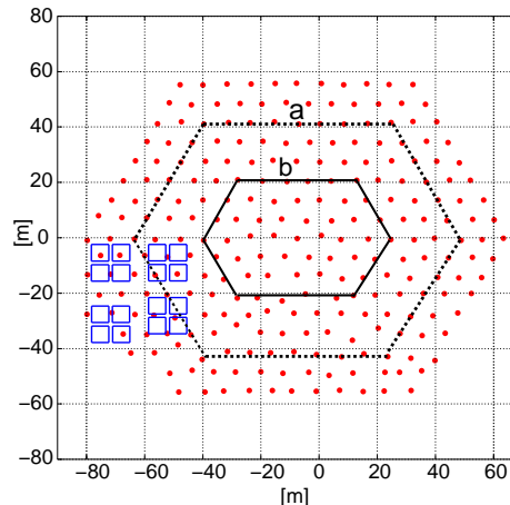
Fig. 1. The GRAPES-3 experimental system with 257 scintillator detectors and 16 muon detector modules
