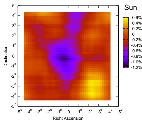
Fig. 5. (a) A 2-D map of % variation in number of showers around the Sun. The map is centred on the Sun and covers \pm 5^\circ in R.A. and declination. A significant decrease seen in a region of \sim 2^\circ \times 2^\circ around the Sun.
