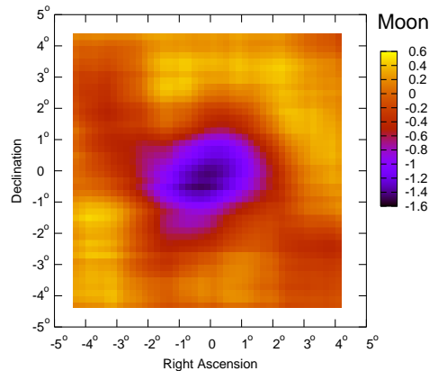
Fig. 4. (a) A 2-D map of % variation in number of showers from the directions around the Moon. The map is centred on the Moon and covers \pm 5^\circ in R.A. and declination. A significant decrease is seen in a region of \sim 1.5^\circ around the Moon.
