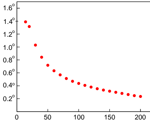
Fig. 2. Variation of the median angle as a function of the number of detectors triggered.
