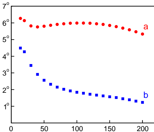
Fig. 3. Variation of the median angle, (a) \alpha_{mp} for plane fit shown by filled circles, (b) \alpha_{mc} for cone fit shown by filled squares, as a function of number of detectors triggered.
