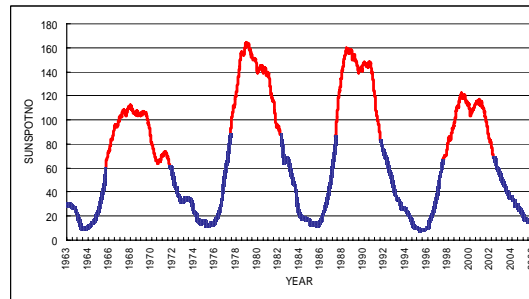
Figure 5: Time profile of the smoothed sunspot numbers after taking the 365-day and 27-day running averages and the definition of the active (red) and quiet (blue) terms of the solar activity.
