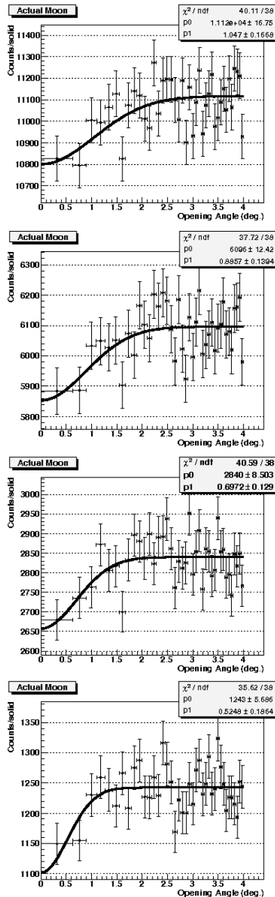
Figure 4: Shadow of the Moon. From top the shower size of \log_{10}(\text{Size}) \geq 3.5 , \geq 3.75 , \geq 4.0 , \geq 4.25 . The angular resolution is 1.05^\circ , 0.89^\circ , 0.70^\circ , 0.52^\circ respectively.
