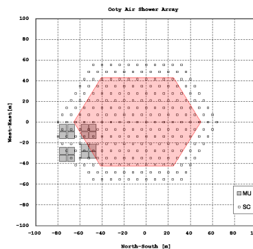
Figure 1: GRAPES-3 air shower array in the period of 2000 - 2003. 256 scintillation detectors and 16 large area muon detectors
