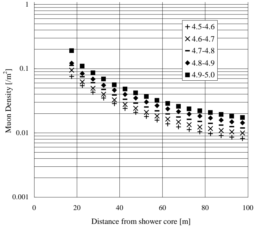
Figure 3: Muon lateral distribution for each shower size groups. ( 5.0 > \log N_e > 4.5 )
