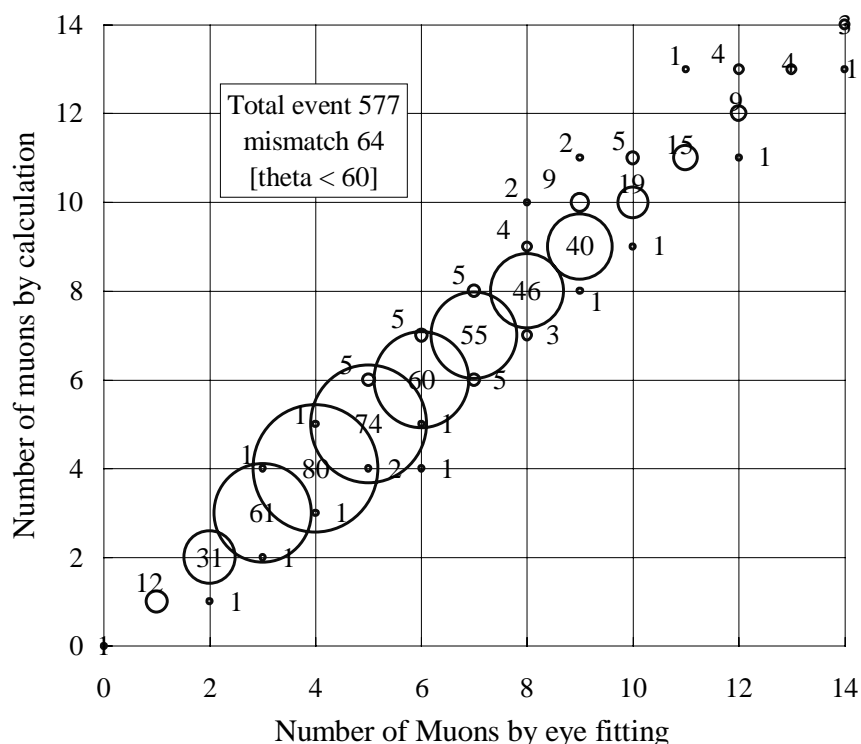
Figure 2: Comparison between eye fitting and automatic calculation for determination of number of Muons[/module]
