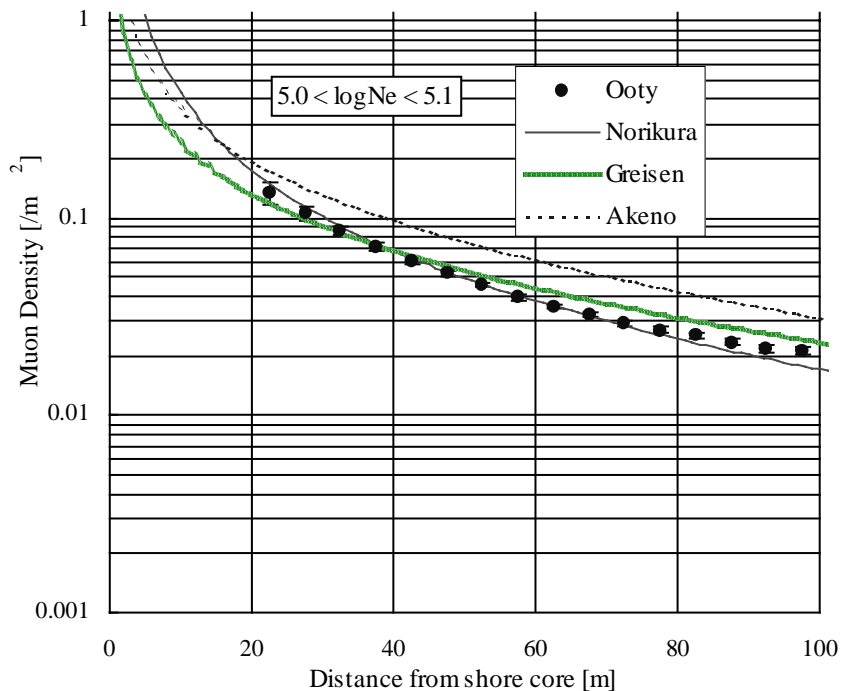
Figure 4: Muon lateral distribution compare with other experimental results.
