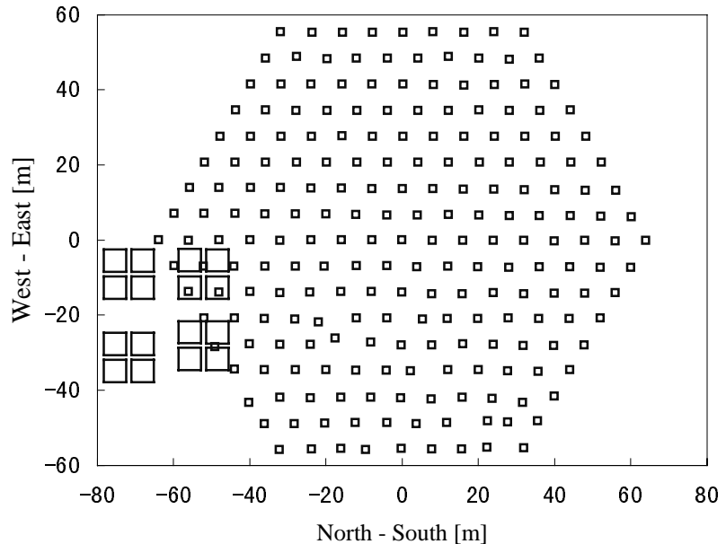
Figure 1: Air Shower Array at Ooty. Small square shows electron detectors, large square shows muon detectors.
