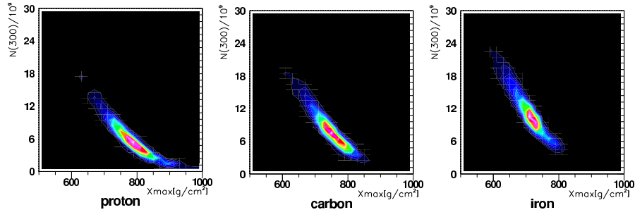
Figure 2. Two dimensional distributions of N_{300} and X_{\max} for reconstructed events which are simulated of primary protons( left ), carbon nuclei( center ), and iron nuclei( right ).
